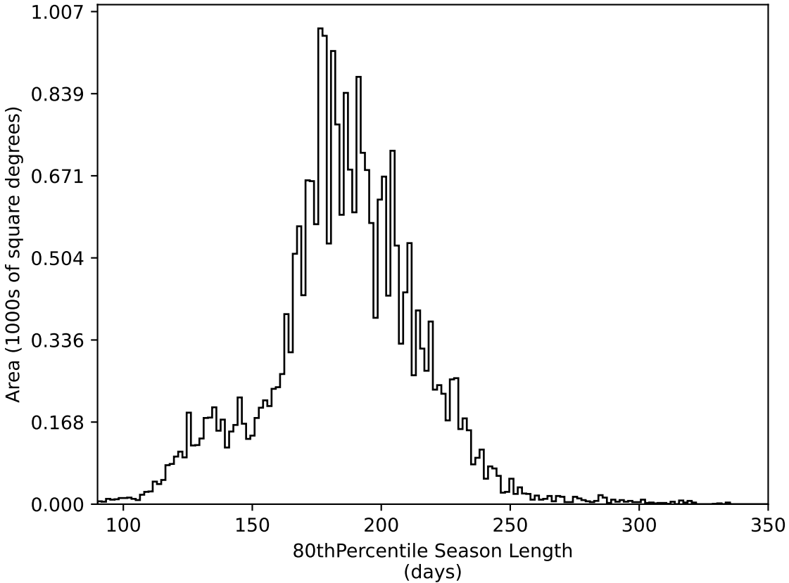
too_elab_2yr_r32_d2_ugrizy_v3.4_10yrs All sky all bands: 80thPercentile Season Length
