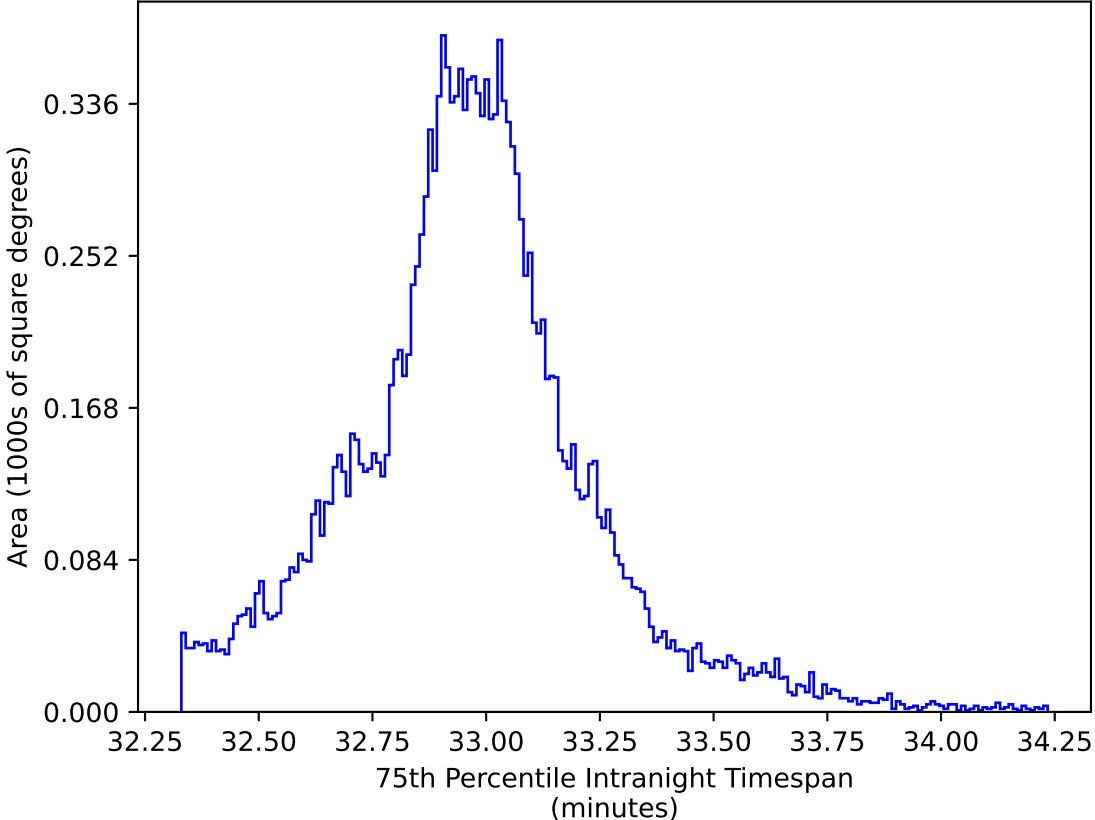
too_elab_2yr_r32_d2_ugrizy_v3.4_10yrs WFD y band: 75th Percentile Intranight Timespan
