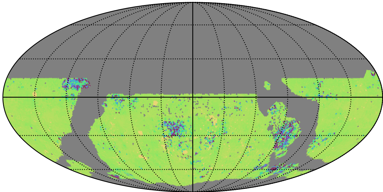
too_elab_2yr_r32_d2_ugrizy_v3.4_10yrs WFD ug bands: 75th Percentile Intranight Timespan
