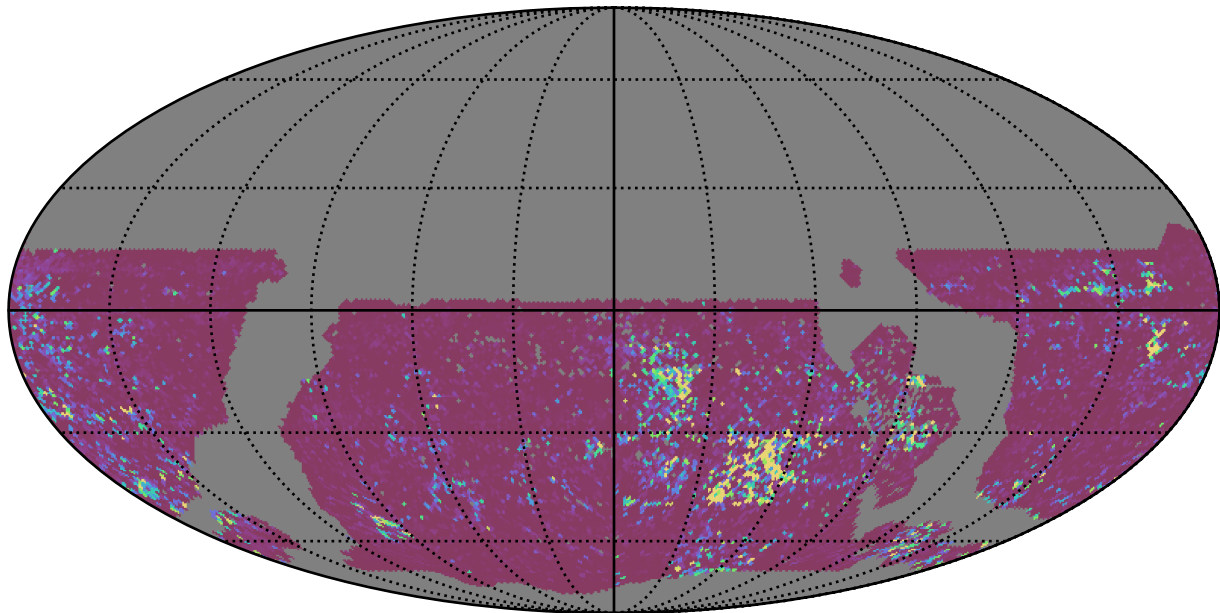
too_elab_2yr_r32_d2_ugrizy_v3.4_10yrs WFD u band: 75th Percentile Intranight Timespan
