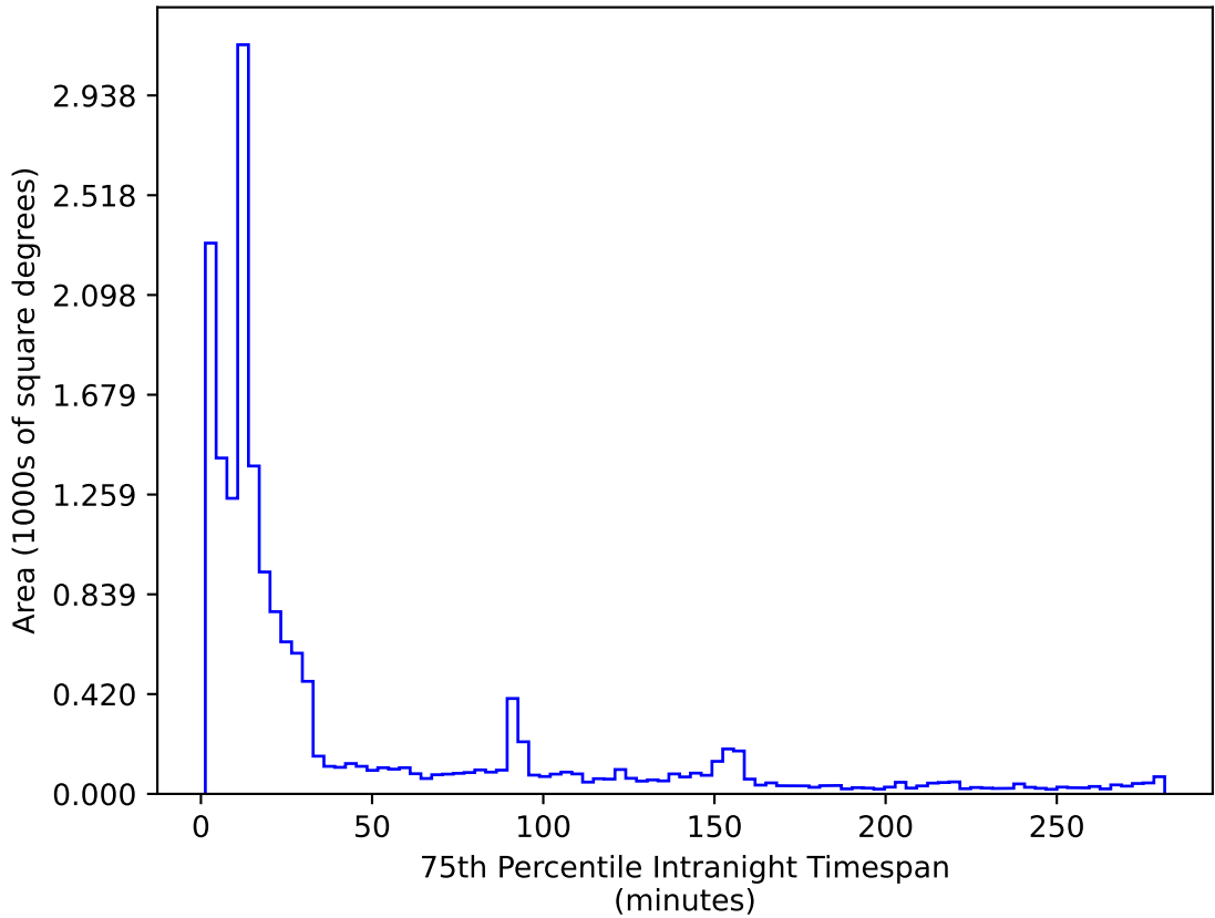
too_elab_2yr_r32_d2_ugrizy_v3.4_10yrs WFD r band: 75th Percentile Intranight Timespan
