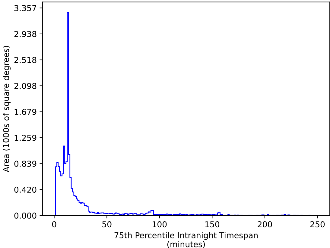
too_elab_2yr_r32_d2_ugrizy_v3.4_10yrs WFD i band: 75th Percentile Intranight Timespan
