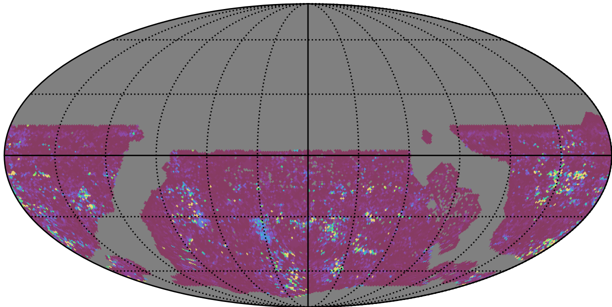
too_elab_2yr_r32_d2_ugrizy_v3.4_10yrs WFD g band: 75th Percentile Intranight Timespan
