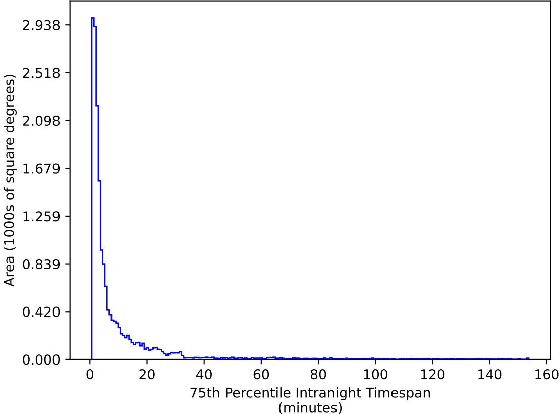
too_elab_2yr_r32_d2_ugrizy_v3.4_10yrs WFD g band: 75th Percentile Intranight Timespan
