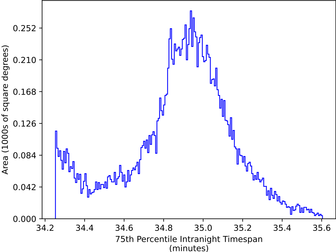
too_elab_2yr_r32_d2_ugrizy_v3.4_10yrs WFD all bands: 75th Percentile Intranight Timespan
