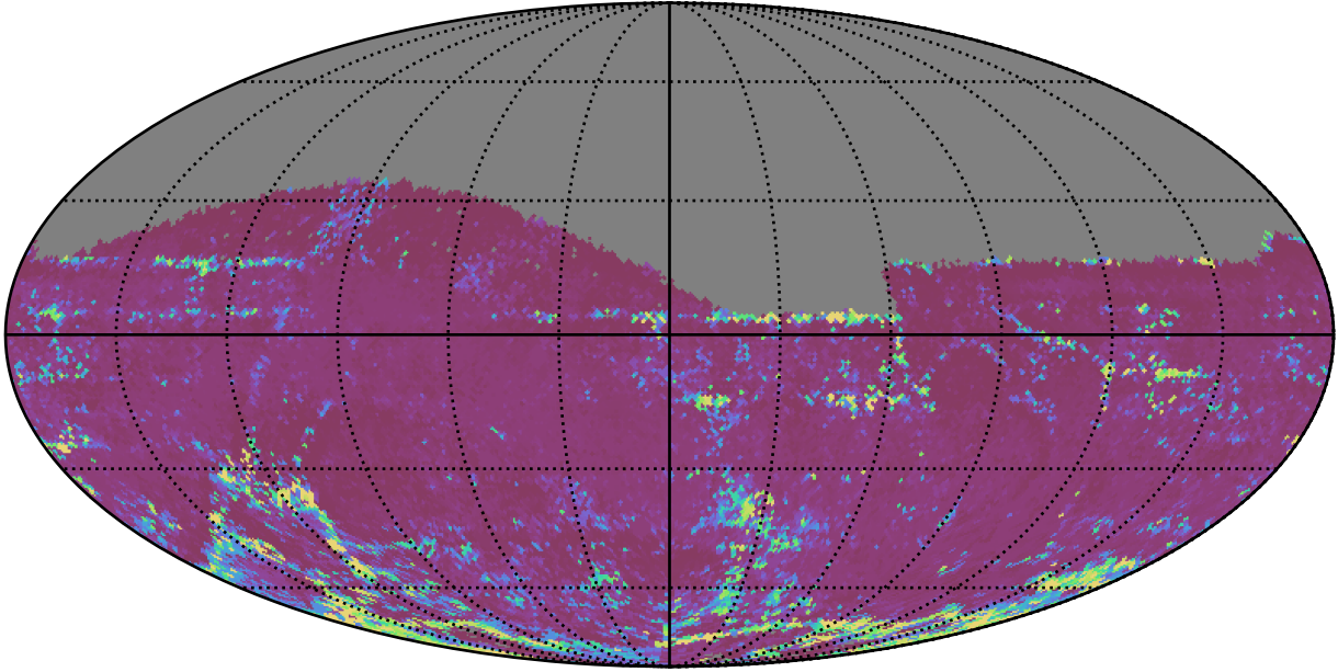
too_elab_2yr_r32_d2_ugrizy_v3.4_10yrs All sky z band: 75th Percentile Intranight Timespan
