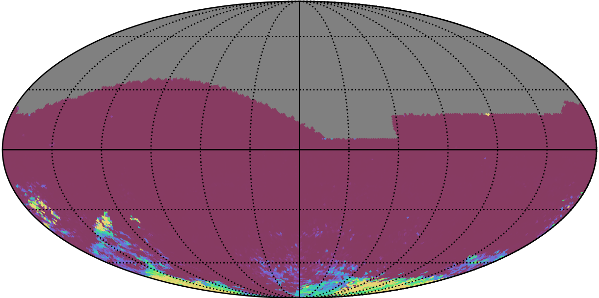
too_elab_2yr_r32_d2_ugrizy_v3.4_10yrs All sky ri bands: 75th Percentile Intranight Timespan
