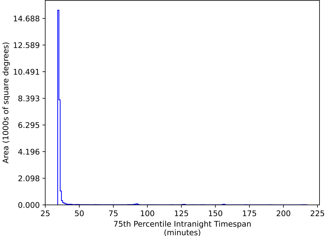
too_elab_2yr_r32_d2_ugrizy_v3.4_10yrs All sky ri bands: 75th Percentile Intranight Timespan
