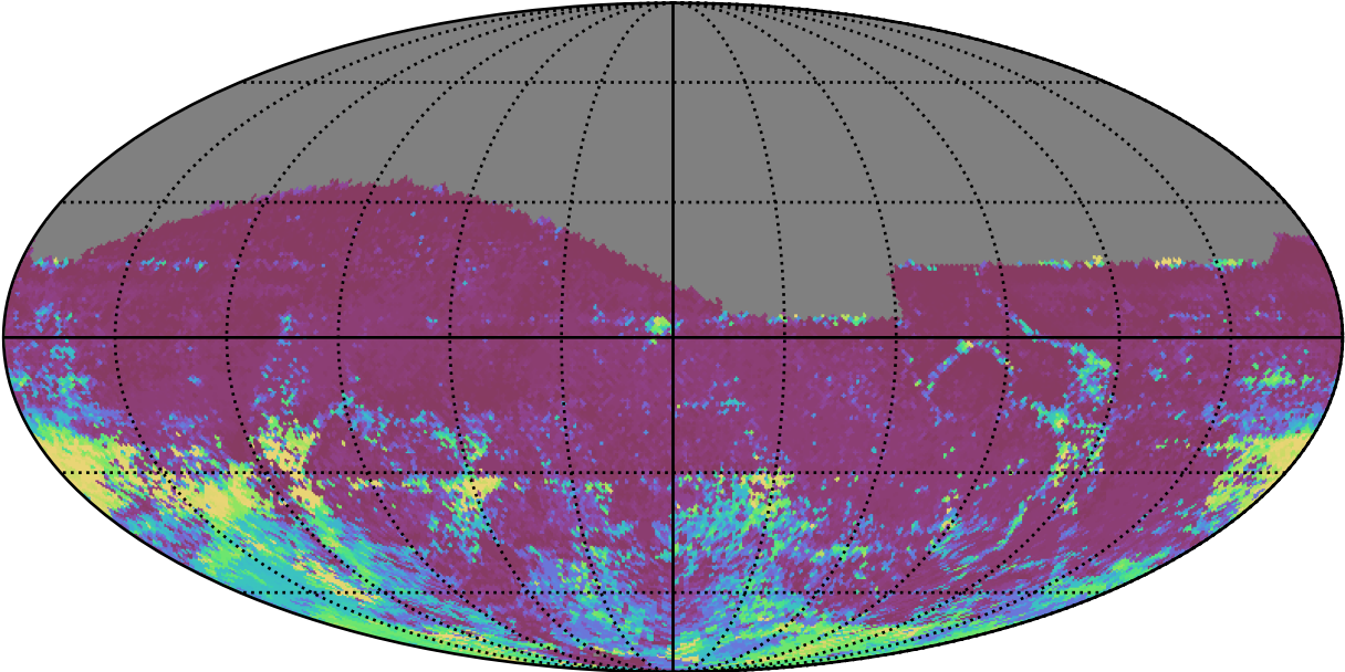
too_elab_2yr_r32_d2_ugrizy_v3.4_10yrs All sky r band: 75th Percentile Intranight Timespan
