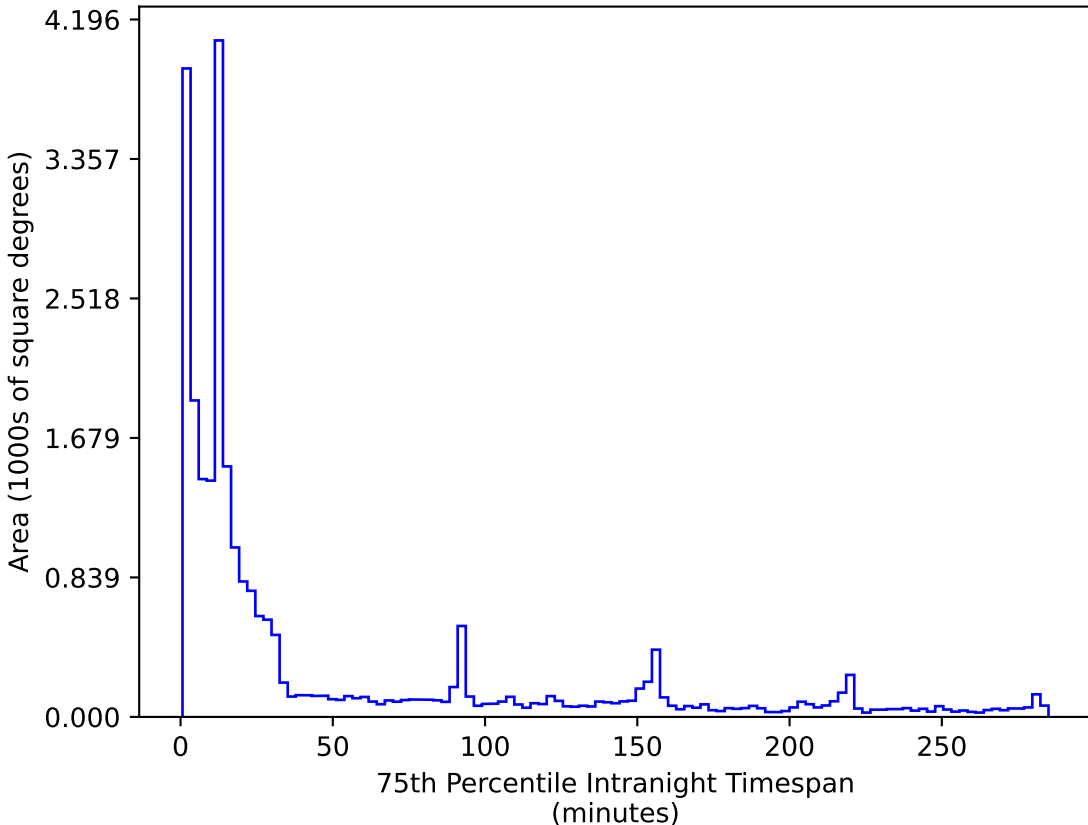
too_elab_2yr_r32_d2_ugrizy_v3.4_10yrs All sky r band: 75th Percentile Intranight Timespan
