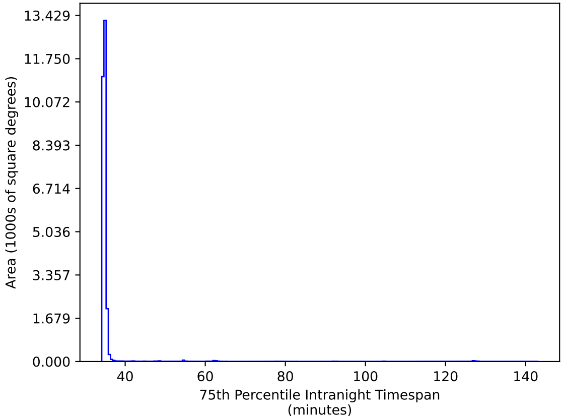
too_elab_2yr_r32_d2_ugrizy_v3.4_10yrs All sky iz bands: 75th Percentile Intranight Timespan
