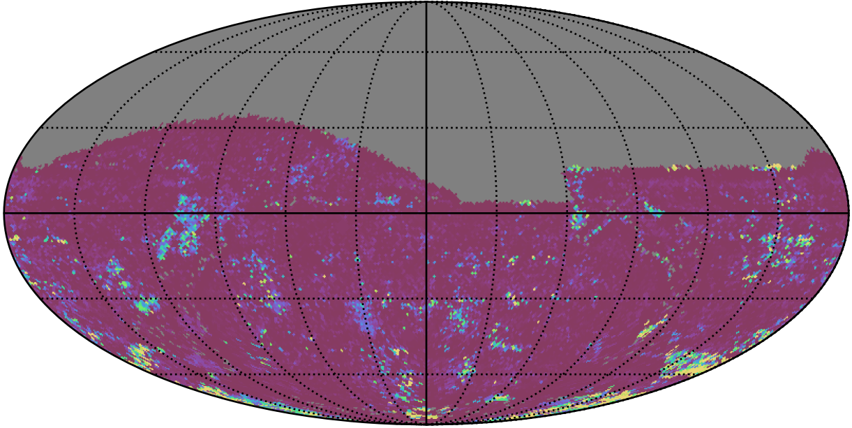
too_elab_2yr_r32_d2_ugrizy_v3.4_10yrs All sky g band: 75th Percentile Intranight Timespan
