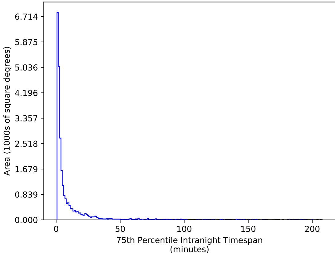
too_elab_2yr_r32_d2_ugrizy_v3.4_10yrs All sky g band: 75th Percentile Intranight Timespan
