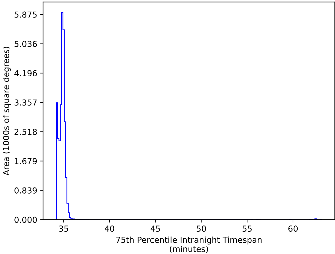
too_elab_2yr_r32_d2_ugrizy_v3.4_10yrs All sky all bands: 75th Percentile Intranight Timespan
