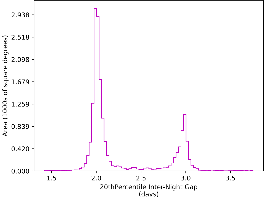
too_elab_2yr_r32_d2_ugrizy_v3.4_10yrs WFD z band: 20thPercentile Inter-Night Gap
