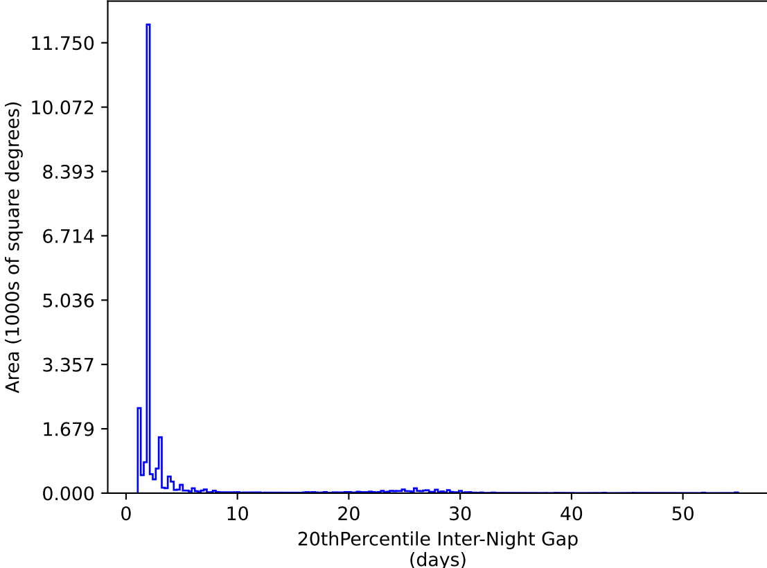
too_elab_2yr_r32_d2_ugrizy_v3.4_10yrs All sky y band: 20thPercentile Inter-Night Gap
