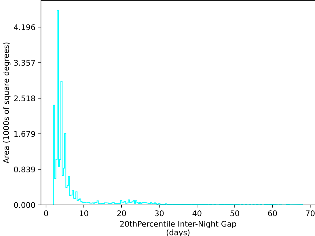
too_elab_2yr_r32_d2_ugrizy_v3.4_10yrs All sky u band: 20thPercentile Inter-Night Gap
