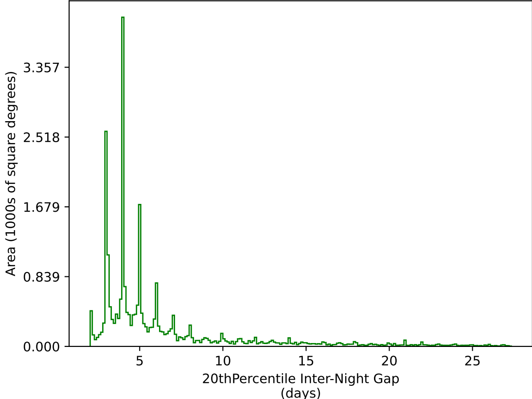
too_elab_2yr_r32_d2_ugrizy_v3.4_10yrs All sky g band: 20thPercentile Inter-Night Gap
