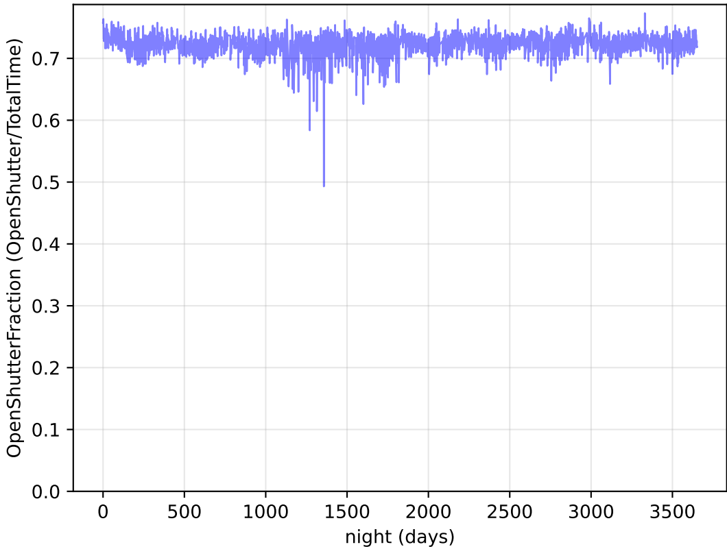
too_elab_2yr_r32_d2_ugrizy_v3.4_10yrs : OpenShutterFraction
