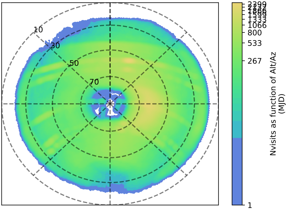
too_elab_2yr_r32_d2_ugrizy_v3.4_10yrs z: Nvisits as function of Alt/Az
