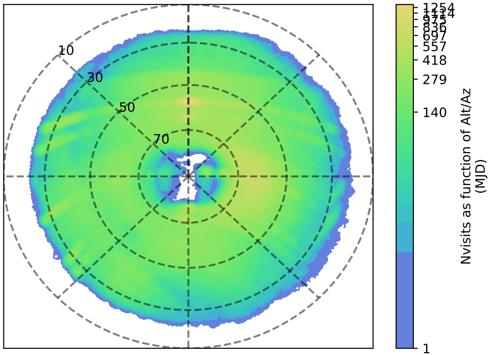
too_elab_2yr_r32_d2_ugrizy_v3.4_10yrs g: Nvisits as function of Alt/Az
