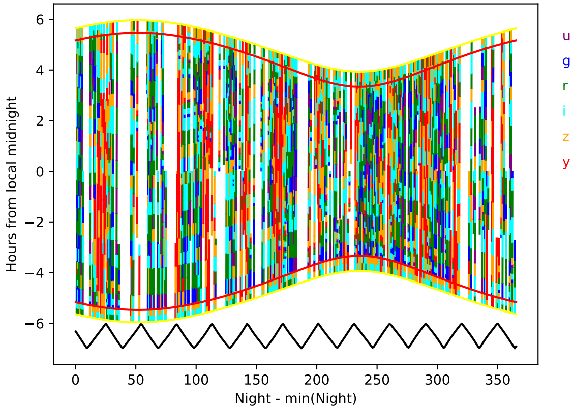
too_elab_2yr_r32_d2_ugrizy_v3.4_10yrs year 7-8: Hourglass
