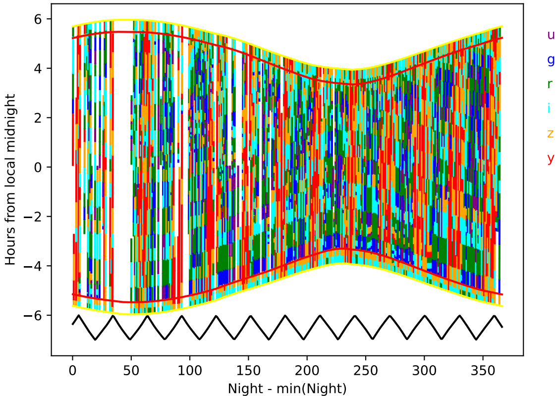
too_elab_2yr_r32_d2_ugrizy_v3.4_10yrs year 6-7: Hourglass
