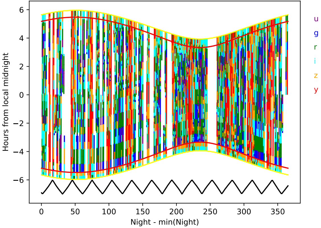
too_elab_2yr_r32_d2_ugrizy_v3.4_10yrs year 5-6: Hourglass
