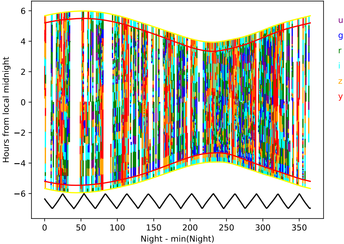
too_elab_2yr_r32_d2_ugrizy_v3.4_10yrs year 4-5: Hourglass
