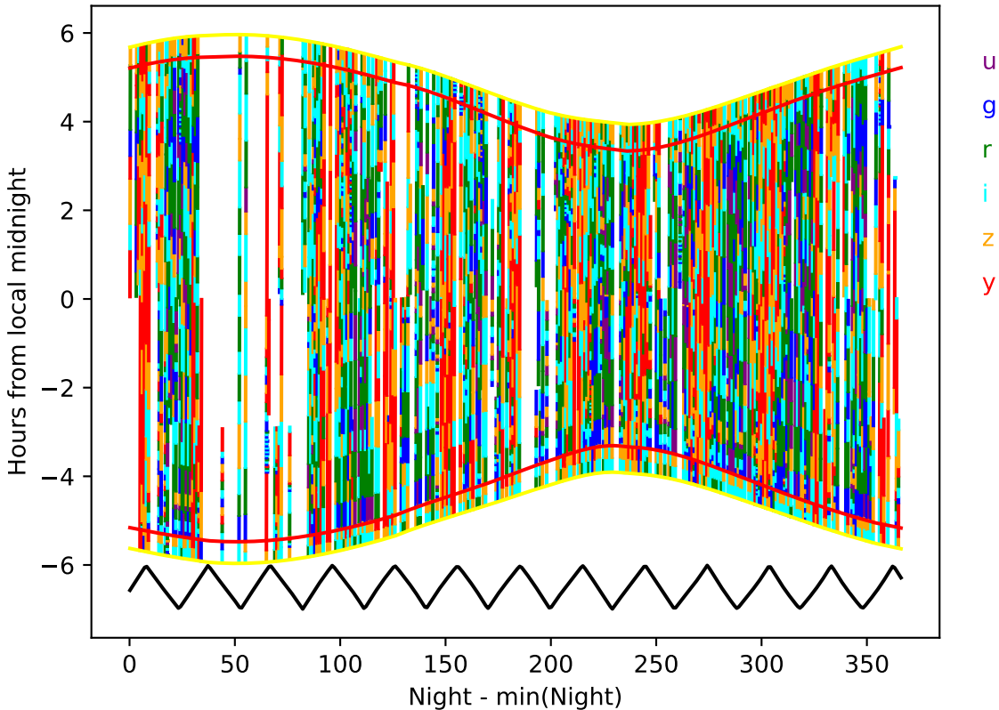
too_elab_2yr_r32_d2_ugrizy_v3.4_10yrs year 3-4: Hourglass
