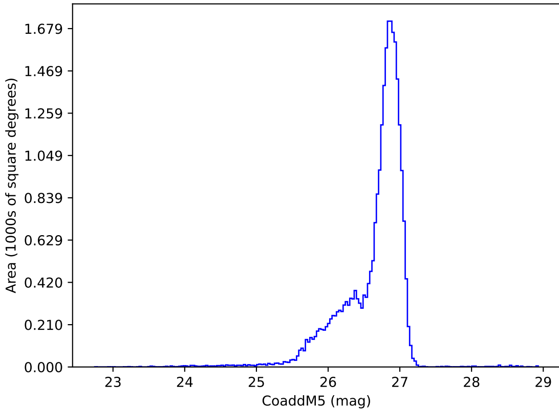
too_elab_2yr_r32_d2_ugrizy_v3.4_10yrs g: CoaddM5
