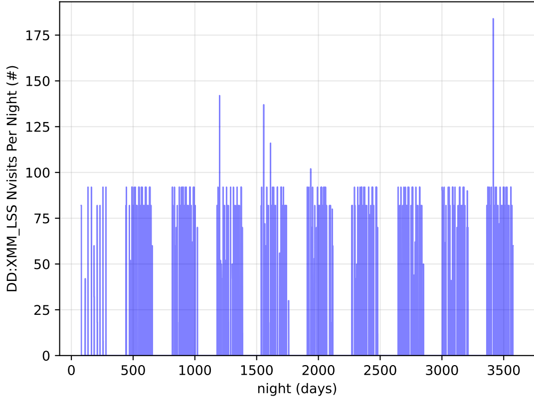
too_elab_2yr_r32_d2_ugrizy_v3.4_10yrs all bands: DD:XMM_LSS Nvisits Per Night
