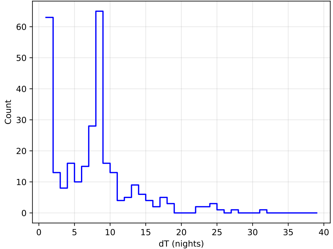
too_elab_2yr_r32_d2_ugrizy_v3.4_10yrs all bands: DD:XMM_LSS Delta Nights Histogram
