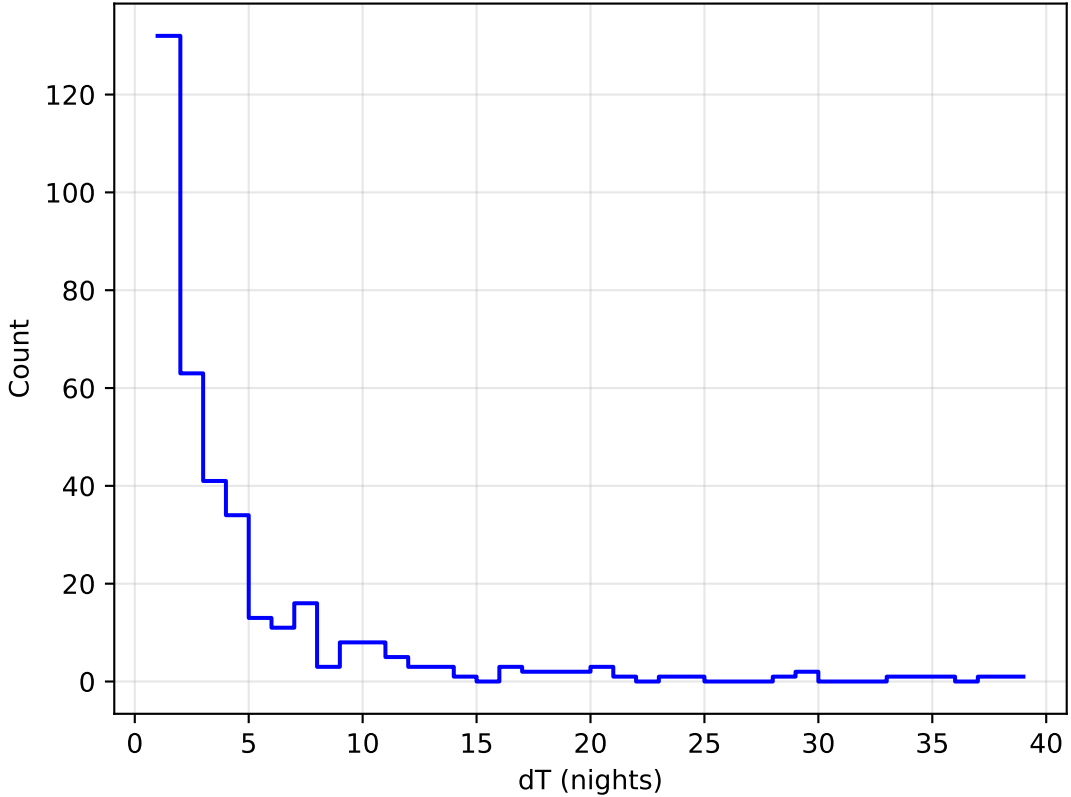
too_elab_2yr_r32_d2_ugrizy_v3.4_10yrs all bands: DD:WFD Delta Nights Histogram
