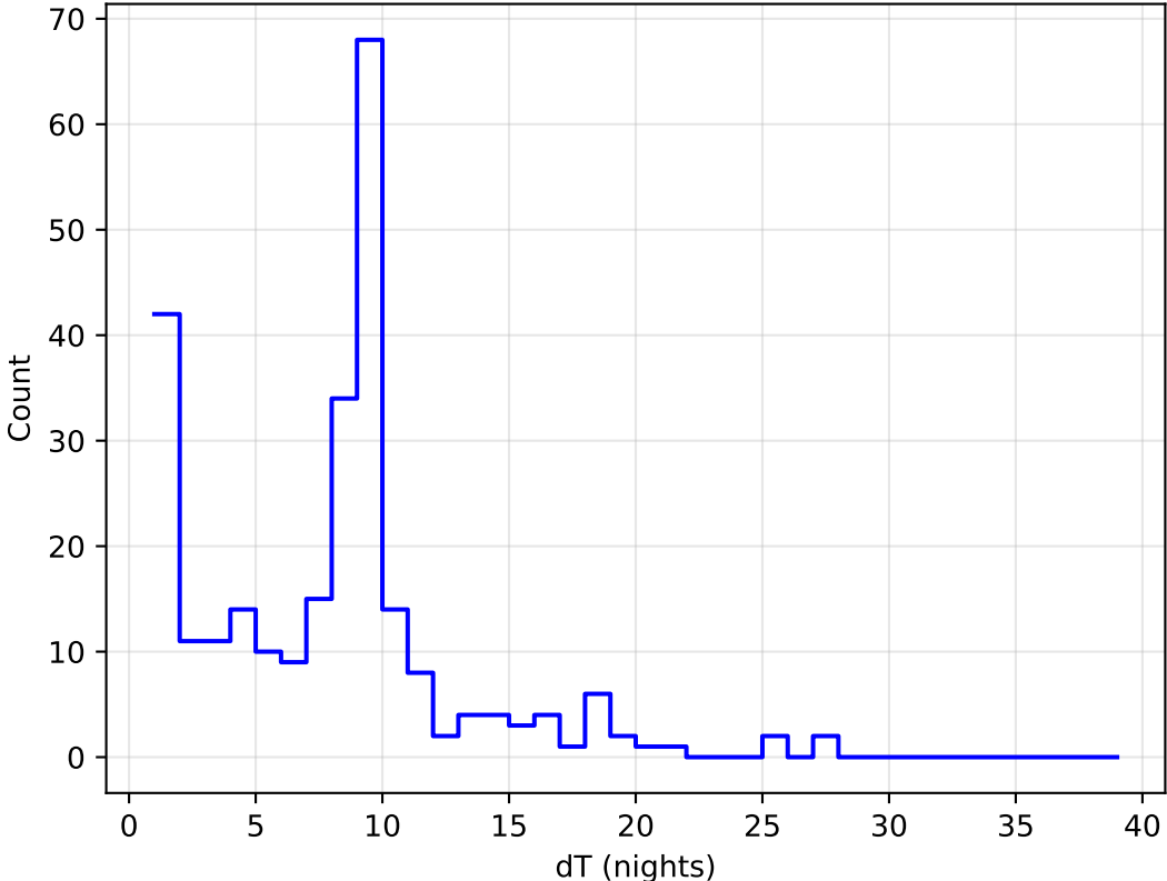
too_elab_2yr_r32_d2_ugrizy_v3.4_10yrs all bands: DD:ELAISS1 Delta Nights Histogram
