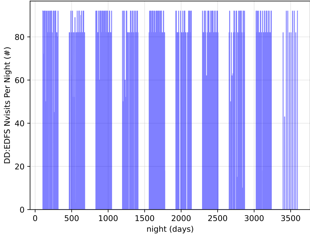
too_elab_2yr_r32_d2_ugrizy_v3.4_10yrs all bands: DD:EDFS Nvisits Per Night
