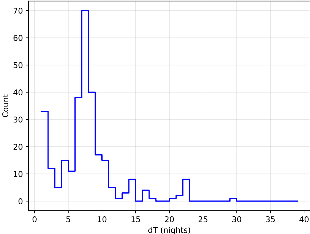
too_elab_2yr_r32_d2_ugrizy_v3.4_10yrs all bands: DD:EDFS Delta Nights Histogram
