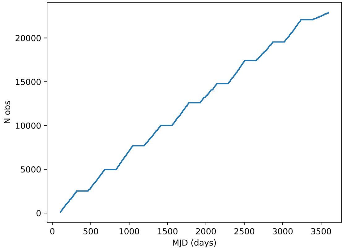
too_elab_2yr_r32_d2_ugrizy_v3.4_10yrs all bands: DD:EDFS Cumulative NVisits
