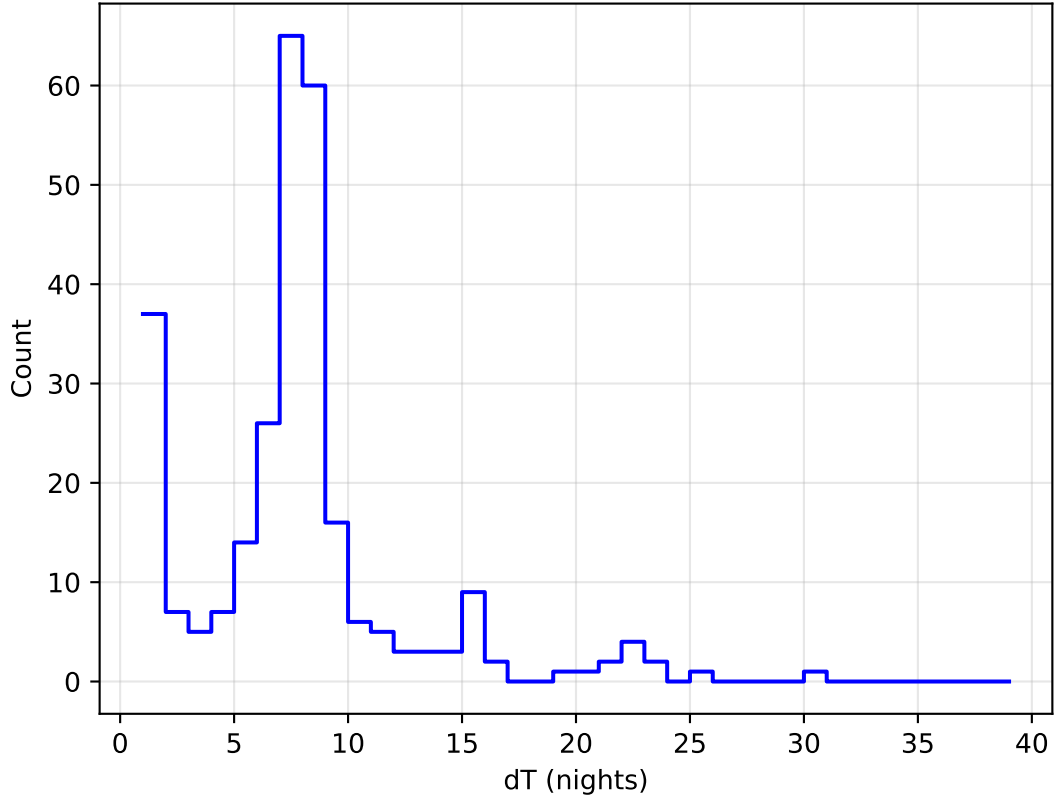
too_elab_2yr_r32_d2_ugrizy_v3.4_10yrs all bands: DD:ECDFS Delta Nights Histogram
