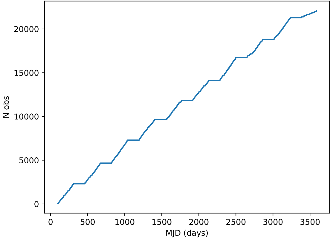
too_elab_2yr_r32_d2_ugrizy_v3.4_10yrs all bands: DD:ECDFS Cumulative NVisits
