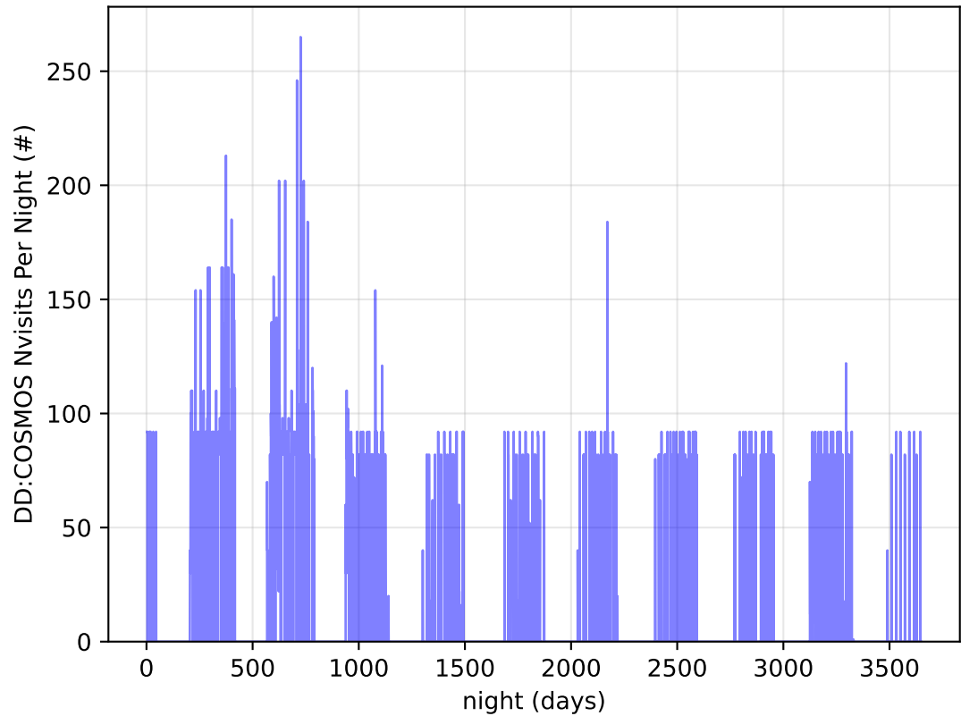
too_elab_2yr_r32_d2_ugrizy_v3.4_10yrs all bands: DD: COSMOS Nvisits Per Night
