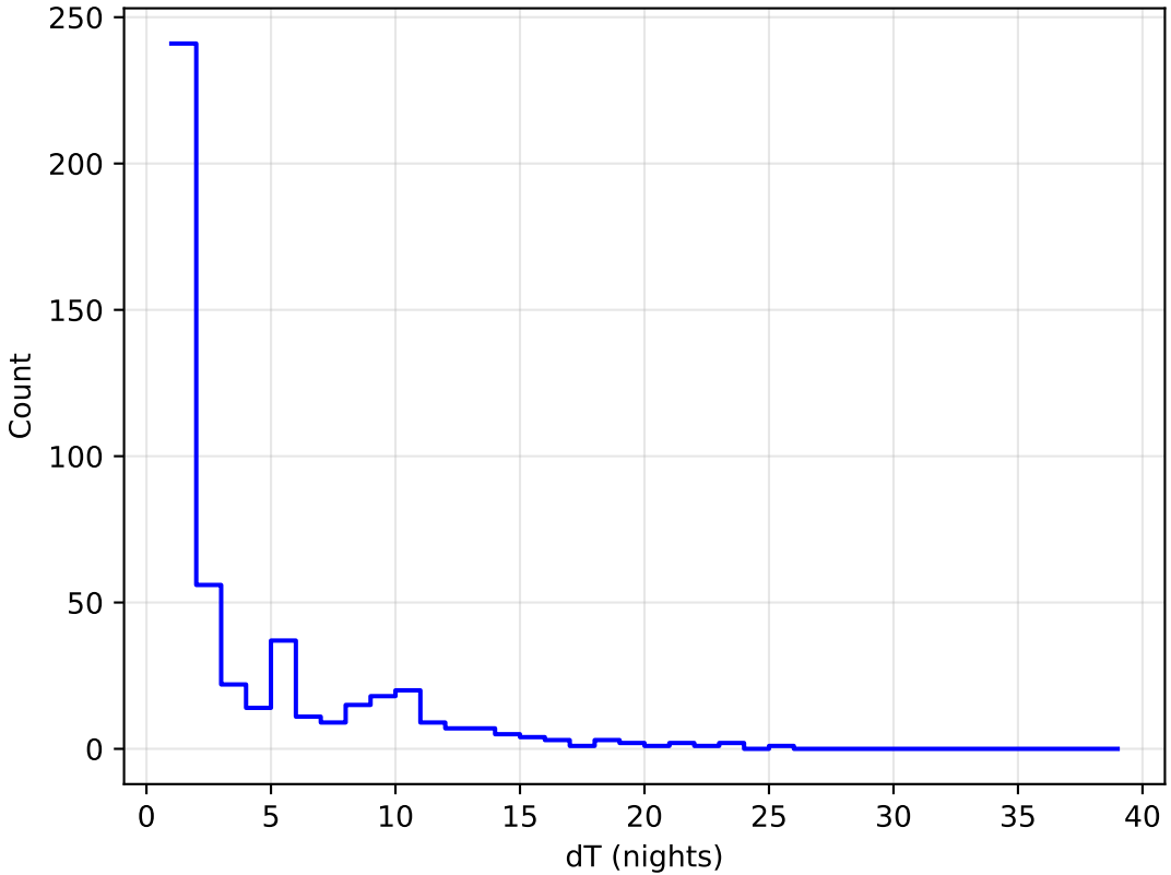
too_elab_2yr_r32_d2_ugrizy_v3.4_10yrs all bands: DD: COSMOS Delta Nights Histogram
