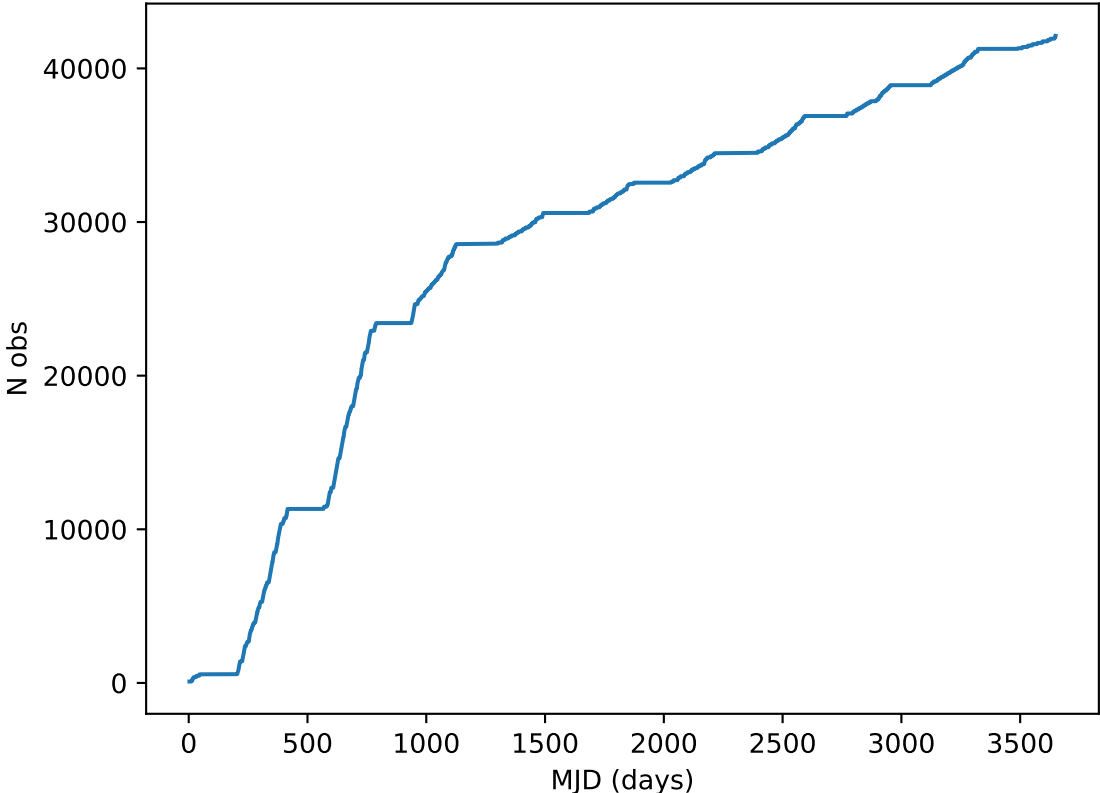
too_elab_2yr_r32_d2_ugrizy_v3.4_10yrs all bands: DD: COSMOS Cumulative NVisits
