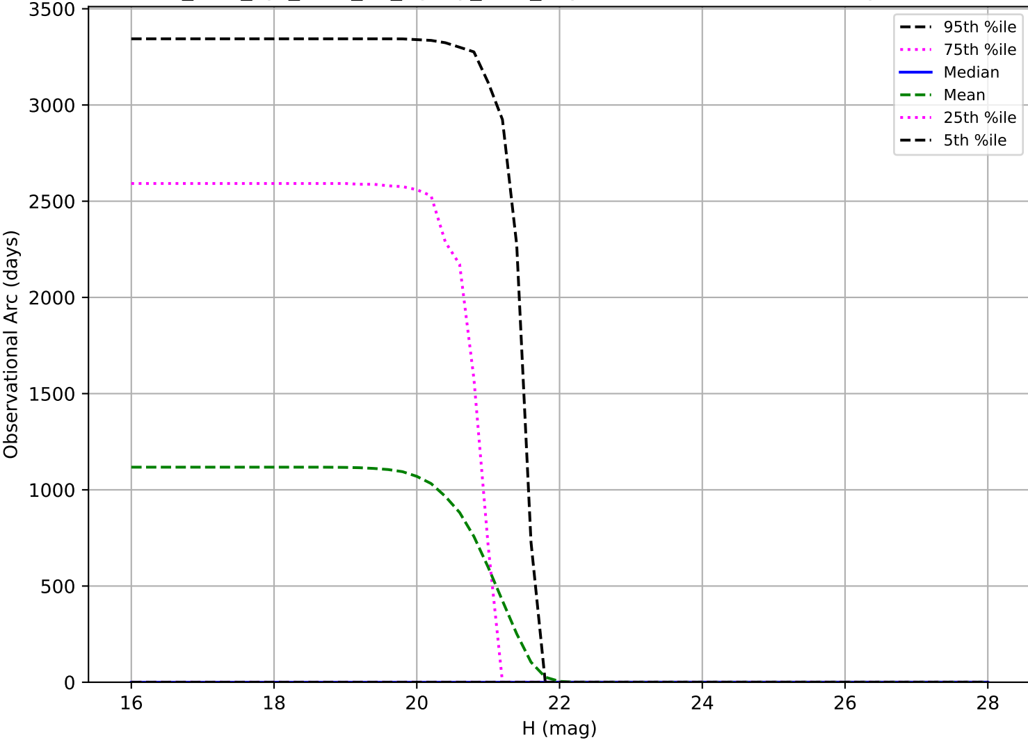
too_elab_2yr_r128_d3_ugrizy_v3.4_10yrs: Observational Arc Length Vatira
