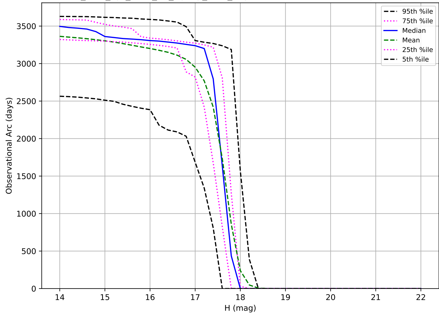
too_elab_2yr_r128_d3_ugrizy_v3.4_10yrs: Observational Arc Length Trojan
