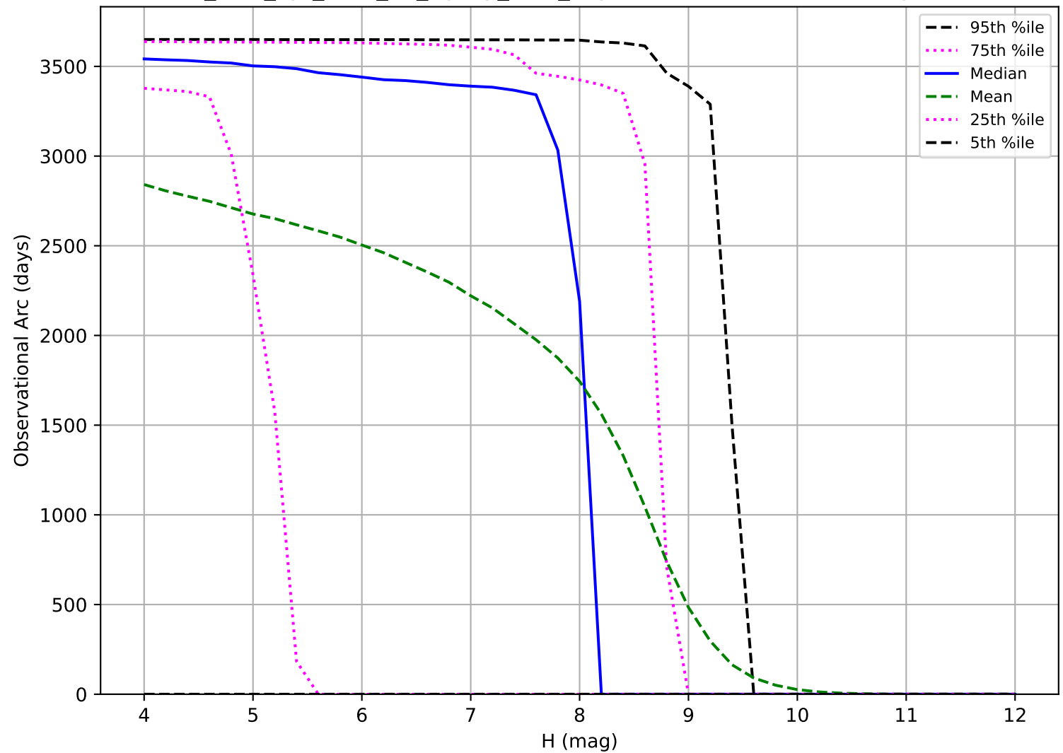
too_elab_2yr_r128_d3_ugrizy_v3.4_10yrs: Observational Arc Length TNO
