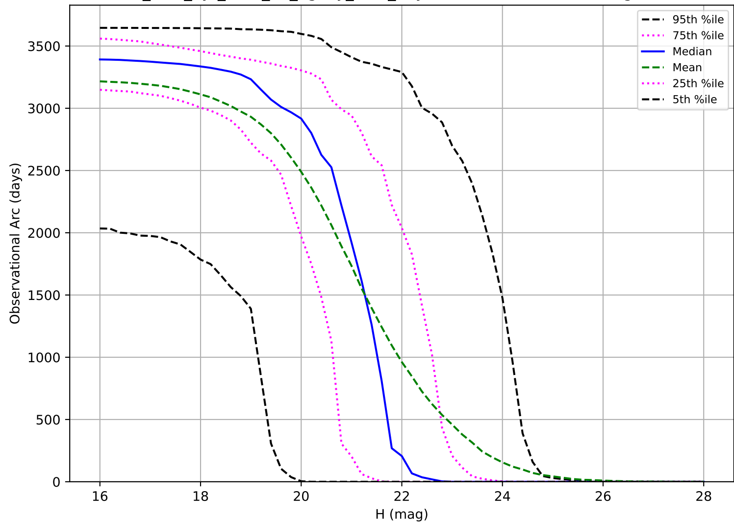
too_elab_2yr_r128_d3_ugrizy_v3.4_10yrs: Observational Arc Length PHA
