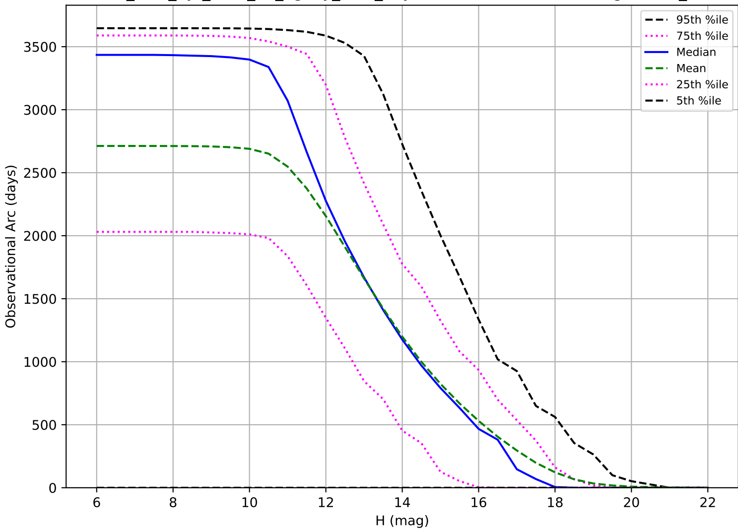
too_elab_2yr_r128_d3_ugrizy_v3.4_10yrs: Observational Arc Length OCC_r5
