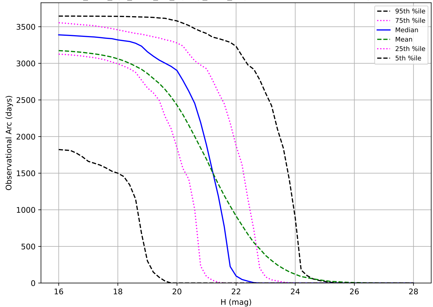
too_elab_2yr_r128_d3_ugrizy_v3.4_10yrs: Observational Arc Length NEO
