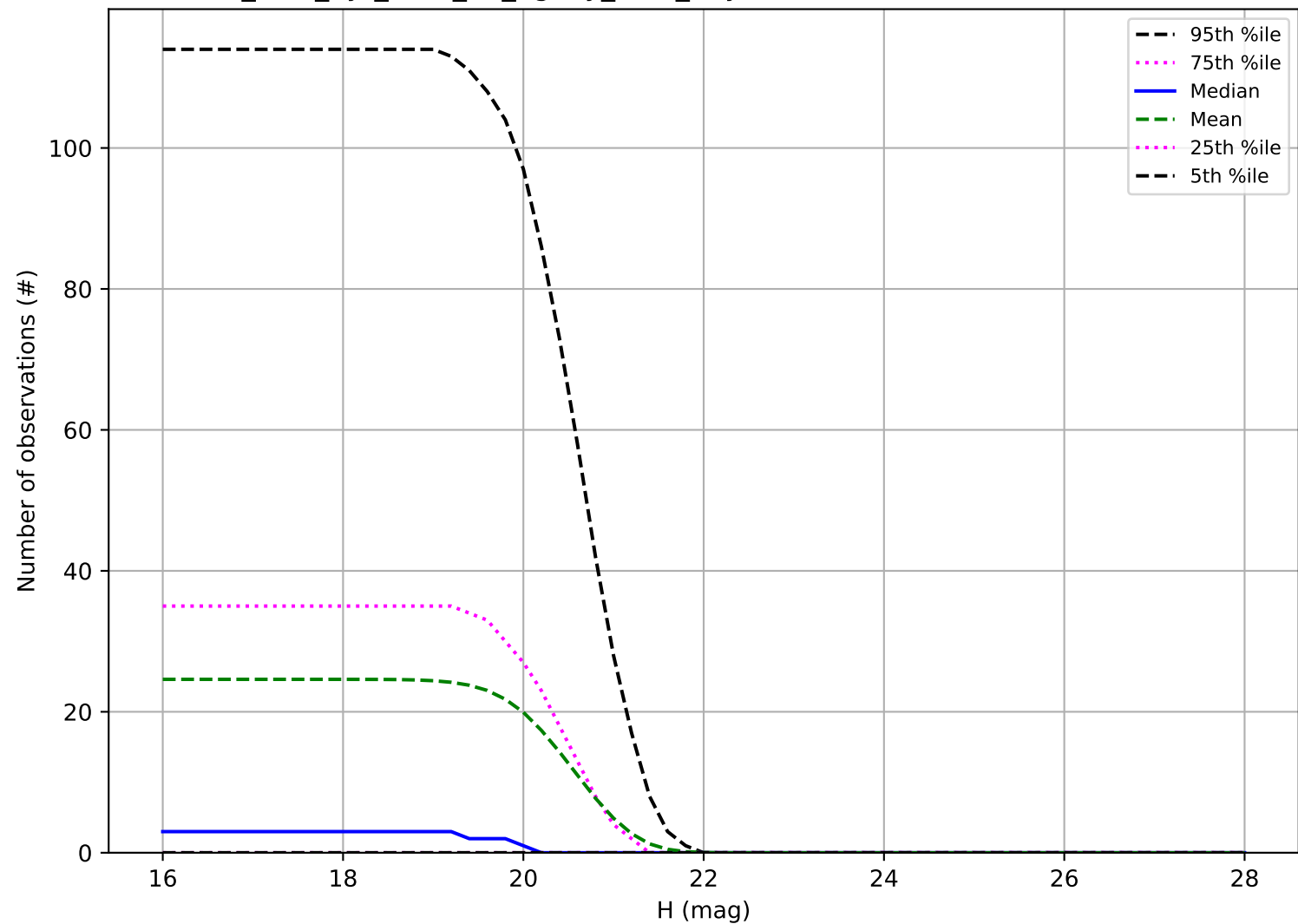
too_elab_2yr_r128_d3_ugrizy_v3.4_10yrs: Number of observations Vatira
